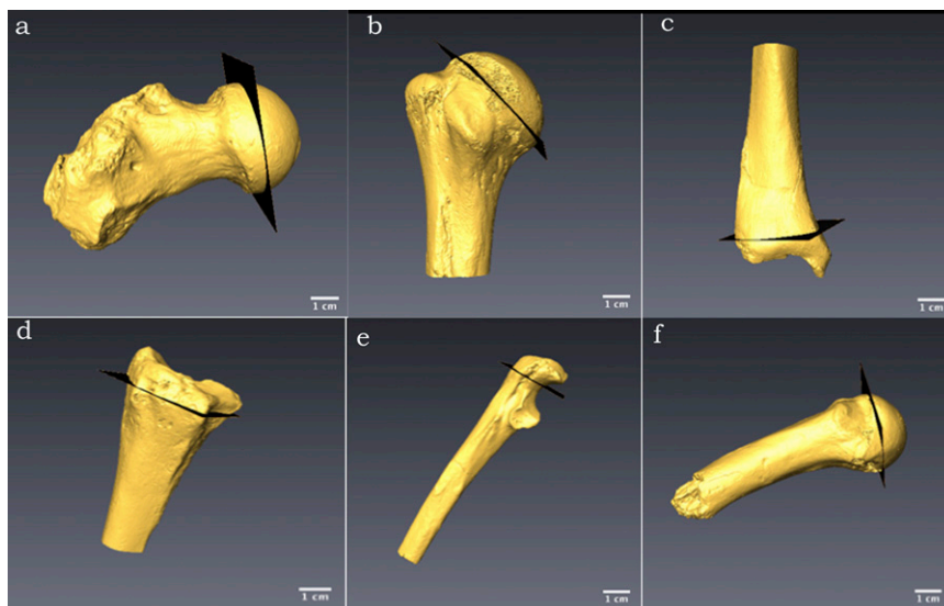
Fig. S2. Images demonstrating the position and plane of the 2D slice in each anatomical element, taken either at the location of pQCT scanning or at a single slice derived from a 3D volume (e.g., in fossil specimens). (A and B) In the femoral head, the medio-lateral breadth is the breadth of the articular surface from the lateral and central-most point of the head to the medial and central-most point of the humeral head (A) and is the breadth of the head from the lateral-most point (including the lesser tuberosity) to the medial and central-most point (B). (C and D) In the distal tibia, the superior–inferior height is measured on the lateral (fibular notch side) surface of the epiphysis, which is the depth of the articulation with the fibula/distal radius, (C) and is measured on the medial side, which is the depth of the articular surface with ulna (D). (E) In the proximal ulna, the superior–inferior height is the height of olecranon process from the most superior border to the center of the trochlear notch. (F) In the metacarpal/metatarsal, the proximal–distal length is measured as the superior–inferior breadth of the head from the central and distal-most point of the head to the proximal extent of the articular surface.
