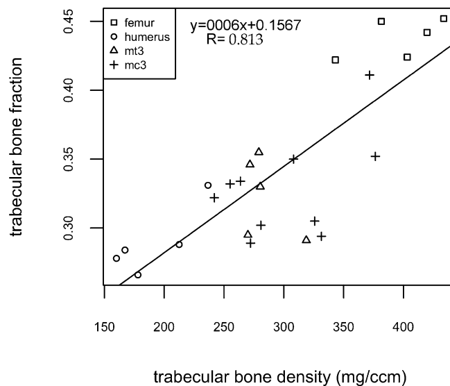
Fig. 55. Plot of the trabecular fraction (bone pixels/total pixels) in chimpanzee femoral ( n = 5 ), humeral ( n = 5 ), metatarsal (mt3; n = 5 ), and metacarpal (mc3; n = 10 ) heads of specimens scanned at the MPI using microCT, against pQCT density measured at the NMNH. The same individuals were scanned with both scanners to establish the relationship between these measures. The linear regression shown here was significant ( P < 0.001 ; R^2 = 0.66 ) and was used to convert pQCT densities (most of the extant samples) into micro-CT trabecular fraction (most of the fossil samples).
