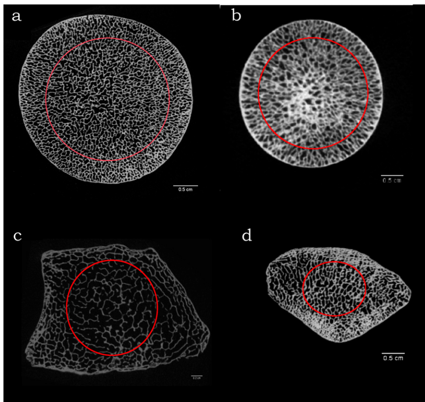
Fig. S1. The ROI in which trabecular fraction was quantified is outlined in red. (A and B) Chimpanzee humeral head (A) and femoral head (B). (C and D) Neanderthal distal radius (C) and proximal ulna (D).
